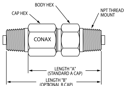
Standard NPT
