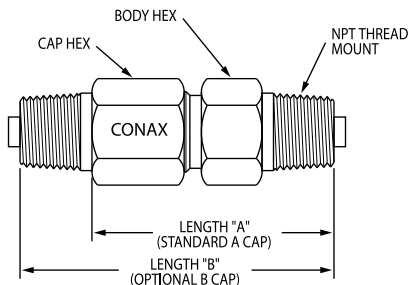
Standard NPT
